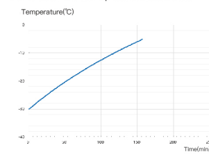
MPR-441FHI Pull-up characteristics
