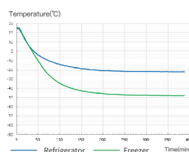
MPR-441FHI Pull-down characteristics
