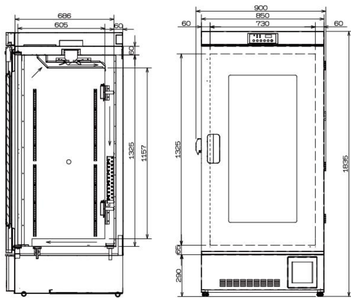
MBR-500 External Dimensions(mm)
