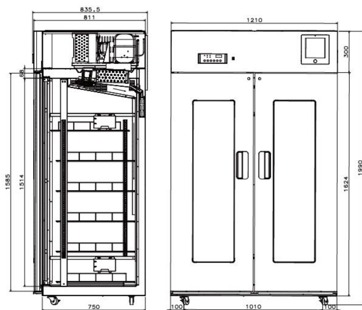
MBR-1000 External Dimensions(mm)
