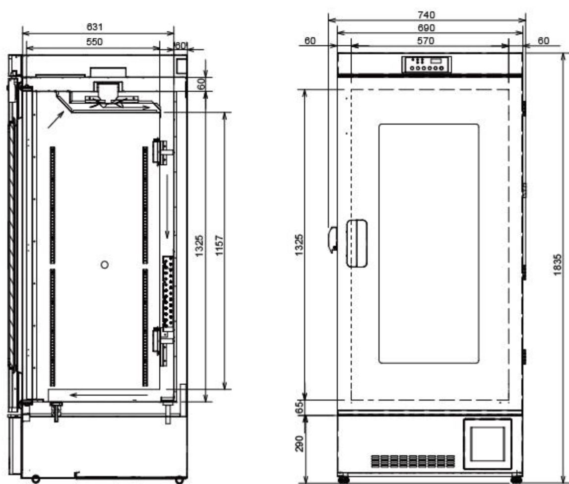
MBR-300 External Dimensions(mm)
